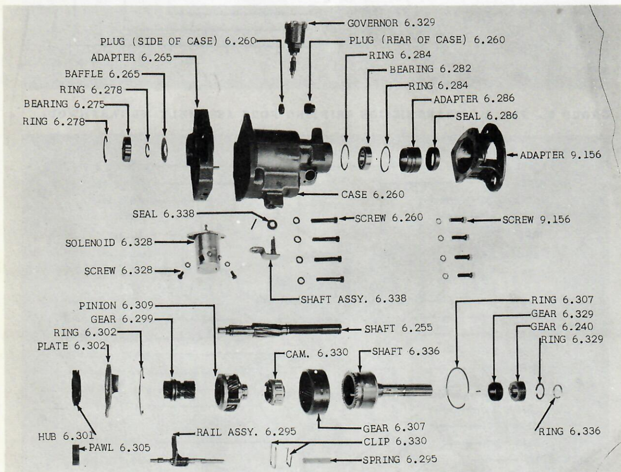
GROUP 6 - FIG. 5 - OVERDRIVE 10-20 (WOD)
