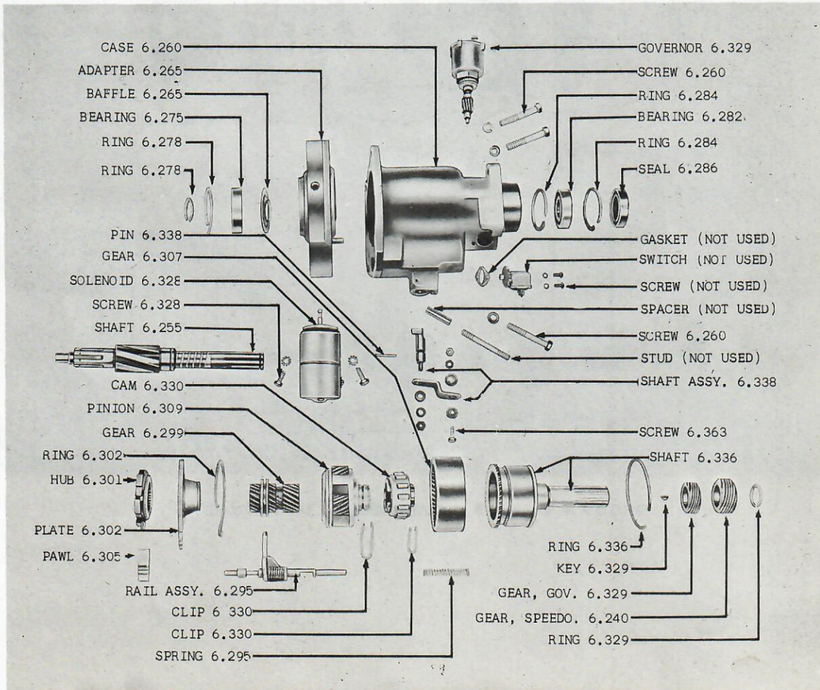
GROUP 6 - FIG. 4 - OVERDRIVE 01 (WOD)
