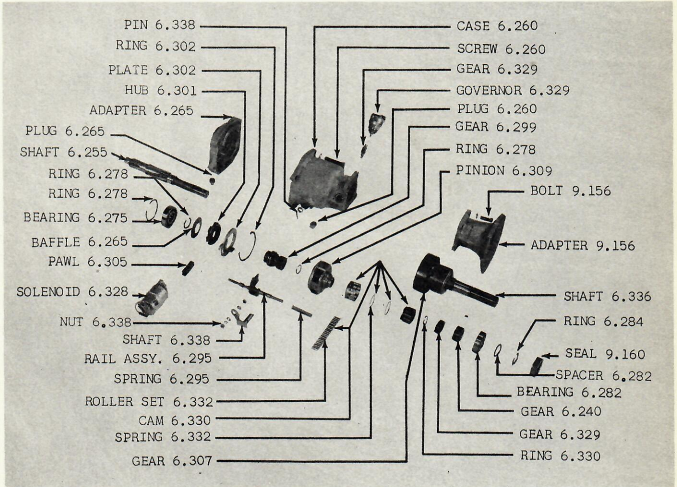
GROUP 6 - FIG. 6 - OVERDRIVE 80 (WOD)
