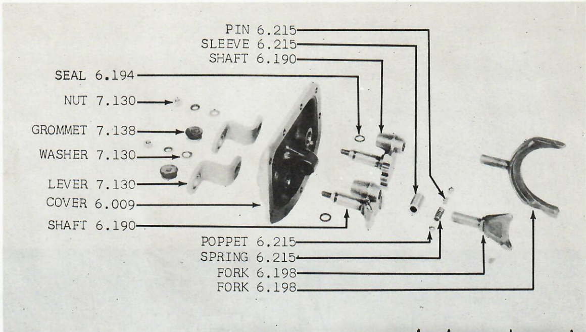
GROUP 6 - FIG. 3 - TRANSMISSION SHIFTING FORK ASSEMBLY 80 (WST)(WOD)
